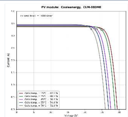
I-V at varying cell temperature (1000 W/m 2 )
