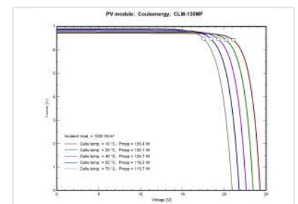
I-V at varying cell temperature (1000 W/m 2 )
